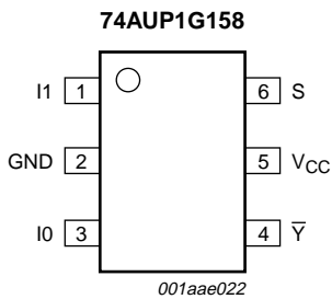
Fig 5. Pin configuration SOT363 (SC-88)
